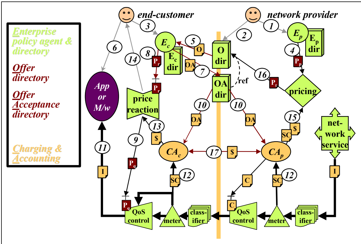
Fig 41 - Dynamic price handler composition
