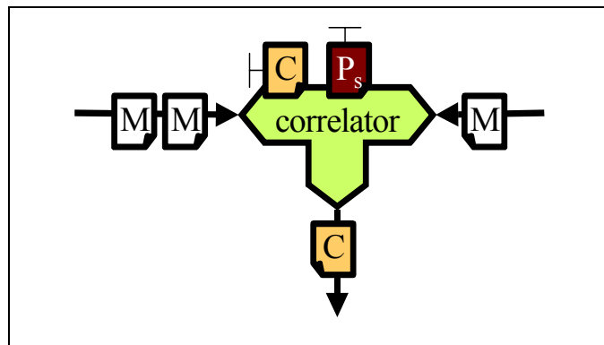
Fig 34 - Correlation
