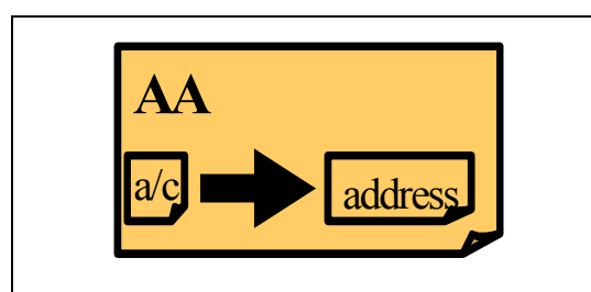
Fig 29 - Address allocation
