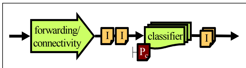
Fig 15 - Classifying
