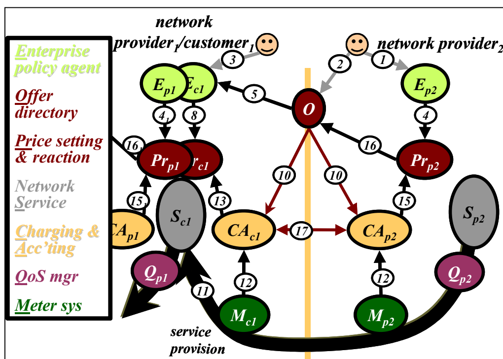
Fig 4 - Inter-network use-case
