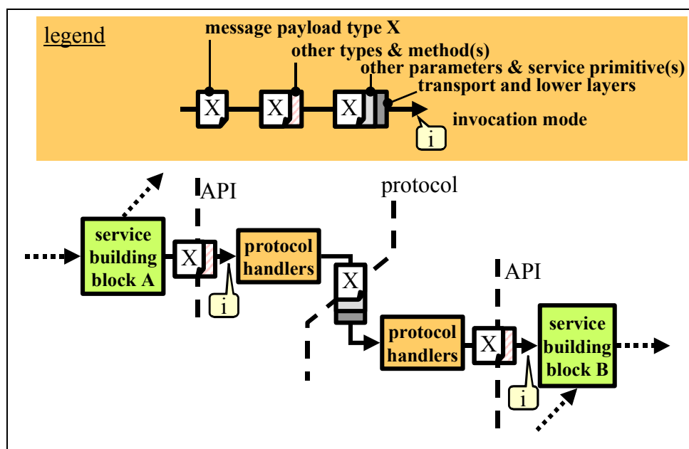
Fig 9 - Interface approach
