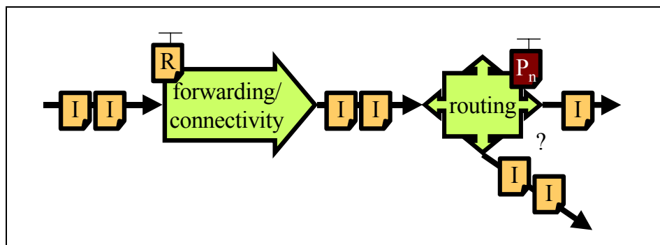
Fig 14 - Networking
