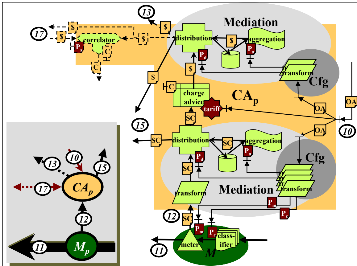
Fig 40 - Charging and accounting service component
