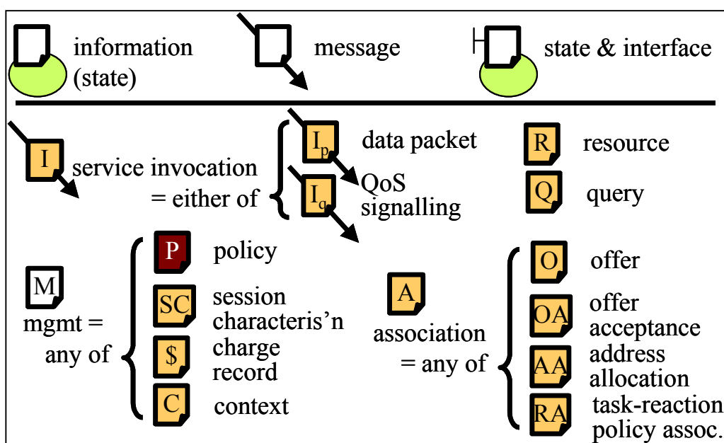
Fig 12 - Legend: state
