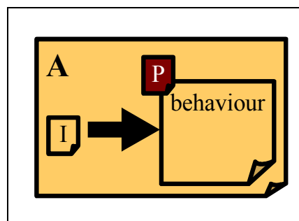
Fig 24 - Service definition
