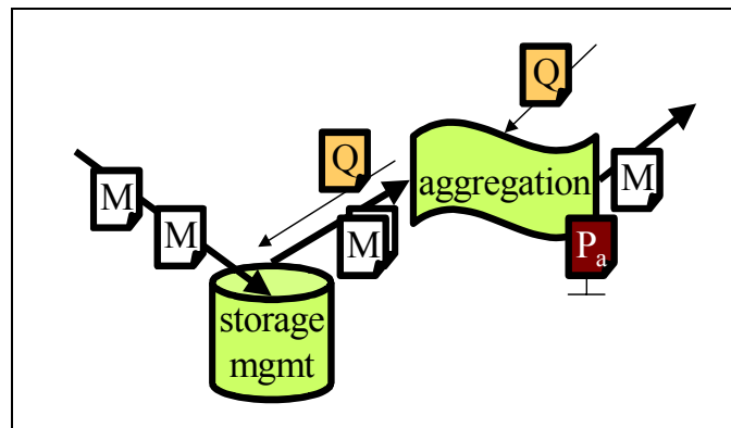
Fig 21 – Aggregation
